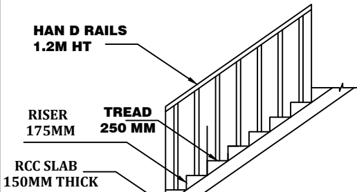
STAIRCASE DETAILS SCALE 1:50
