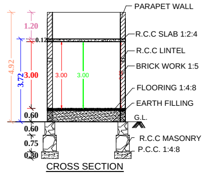
CROSS SECTION
