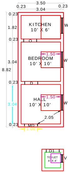
GROUND FLOOR RESIDENTIAL PLAN
