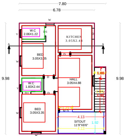
PROPOSED GF PLAN
