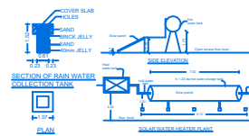
SECTION OF RAIN WATER HARVESTING TANK
