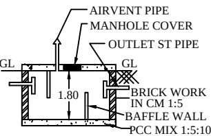
SECTION ON SEPTICTANK
