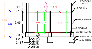
SECTION AB
