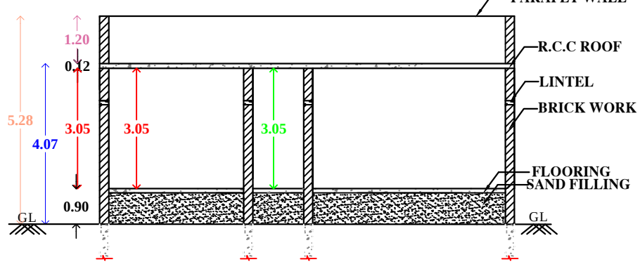
"SECTION "AB"
