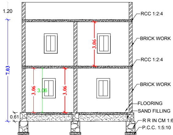
SECTION AB
