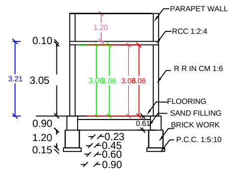
SECTION AB
