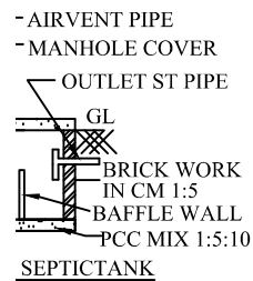
SECTION OF "AB"
