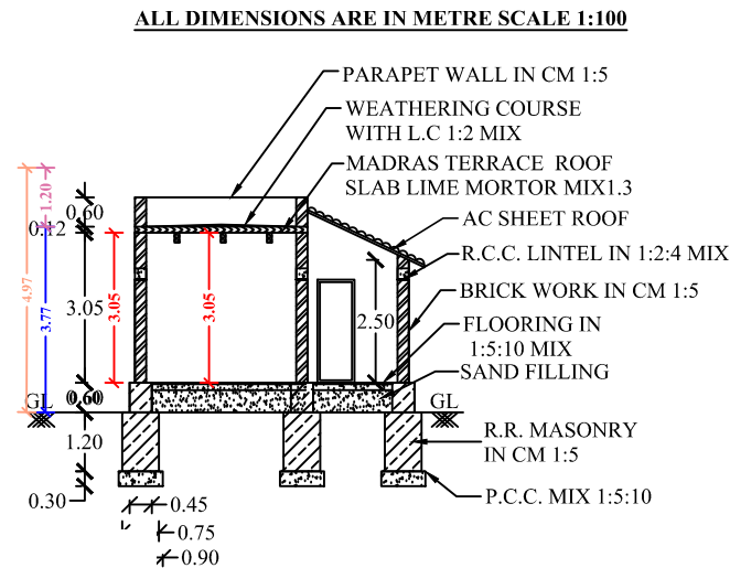
SECTION OF "AB"
