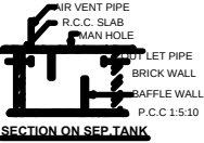
SECTION ON SEP TANK
