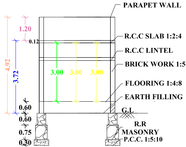
"SECTION "AB"
