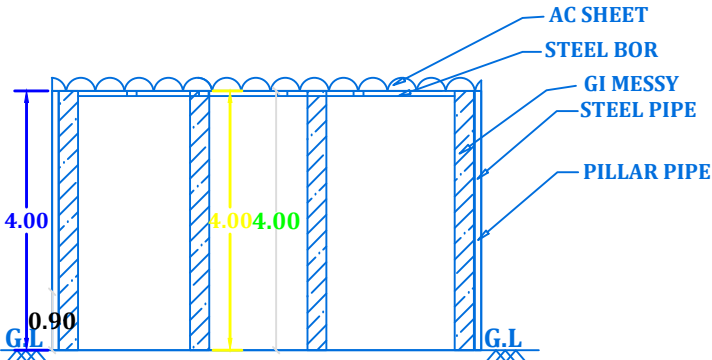
SECTION ON AA1
