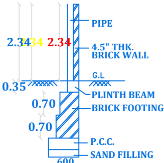
FOUNDATION DETAIL
