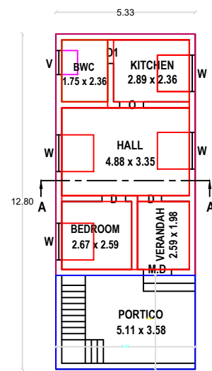
PLAN
