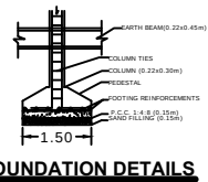
FOUNDATION DETAILS
