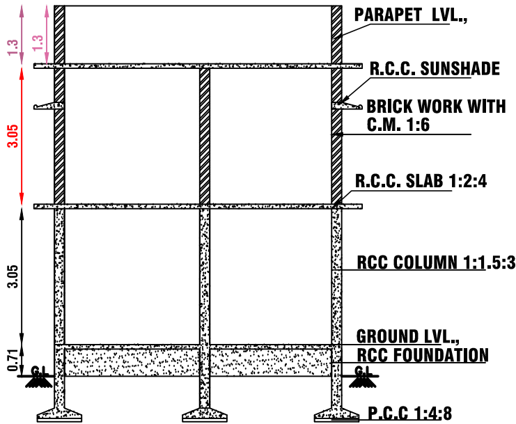
SECTION ON A-A & A'-A'
