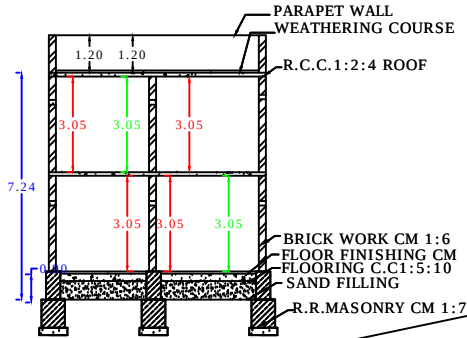
SECTION ON SV
