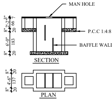
SEPTIC-TANK DETAIL
