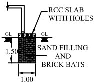
SECTION OF BS
