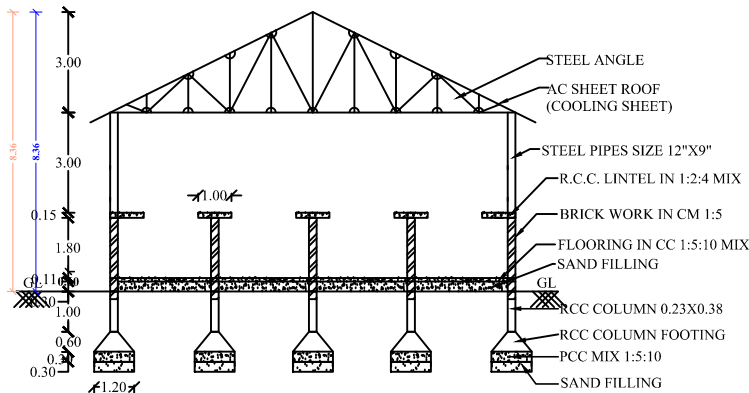
SECTION OF "AB"
