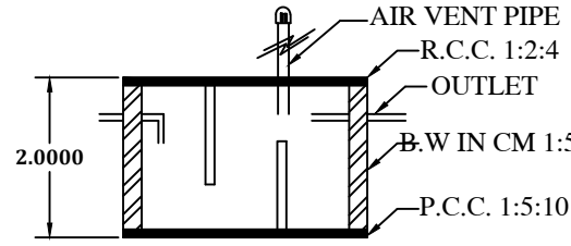
RAIN WATER HARVESTING PIT
