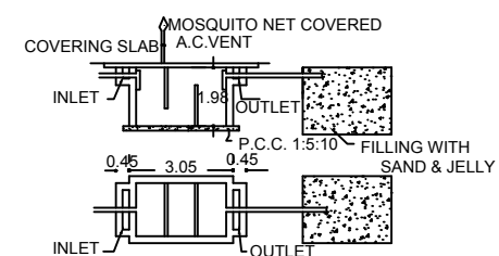
SEPTIC TANK & TRENCH U TRAP PROVISION
