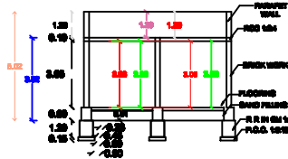
SECTION AB
