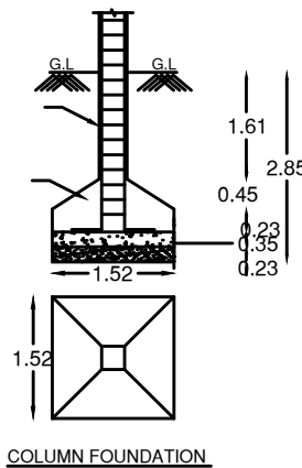
COLUMN FOUNDATION
