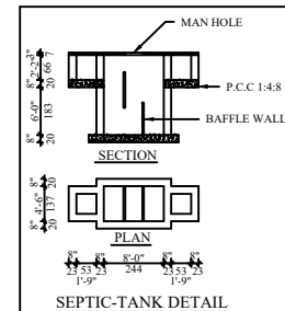
SEPTIC-TANK DETAIL
