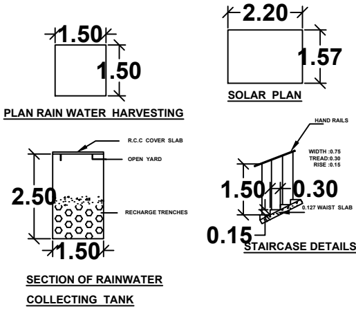
SECTION OF RAINWATER COLLECTING TANK
