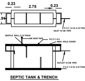
SEPTIC TANK & TRENCH
