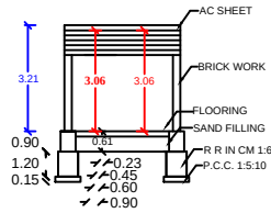
SECTION AB
