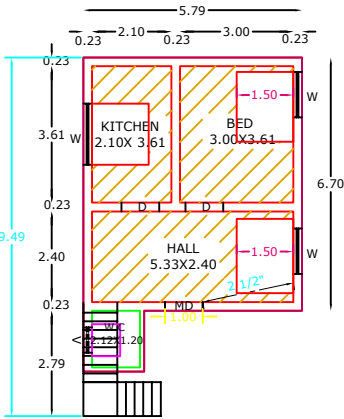
EXT GROUND FLOOR RESIDENTIAL PLAN
