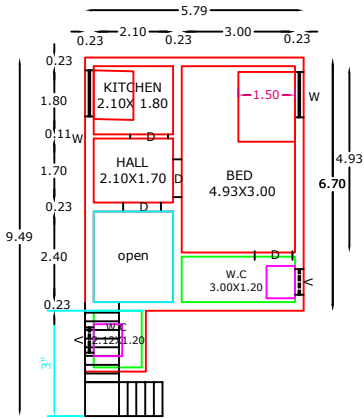
PRO FIRST FLOOR RESIDENTIAL PLAN
