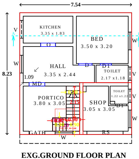
EXG.GROUND FLOOR PLAN
