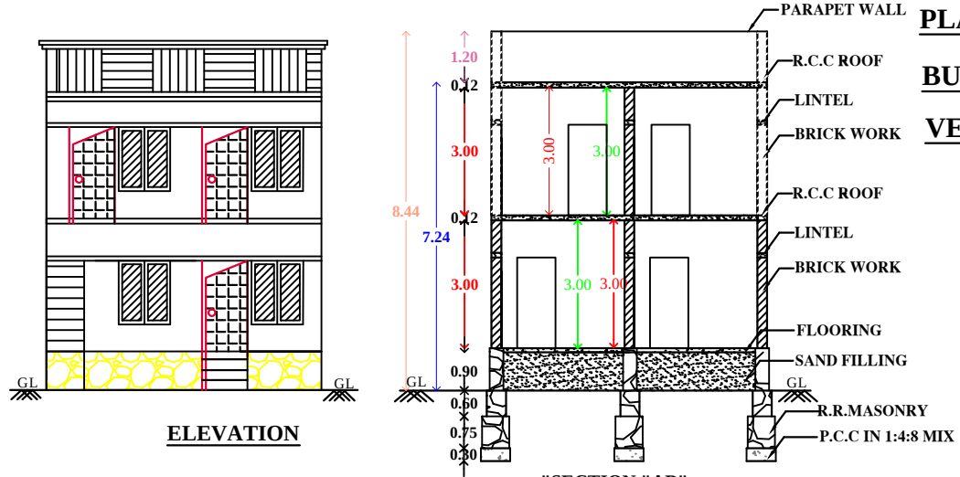
"SECTION AB"
