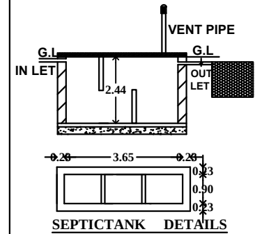
SEPTICTANK DETAILS
