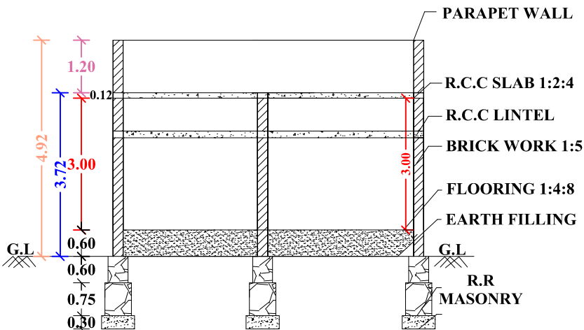
"SECTION "AB"
