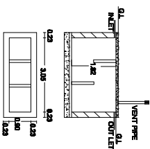
SEPTIC TANK DETAILS
