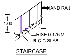
STAIRCASE
