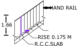
STAIRCASE
