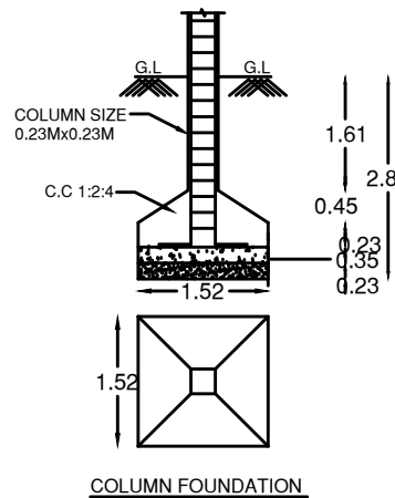
COLUMN FOUNDATION
