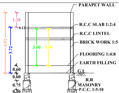
"SECTION "AB"
