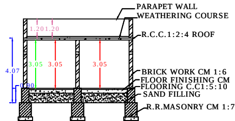
SECTION ON SV
