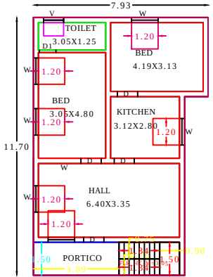
PLAN
