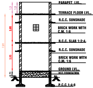
SECTION ON A-A & A'-A'
