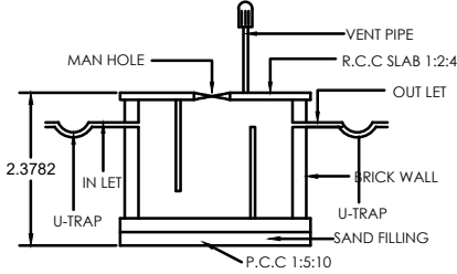
SECTION E,F SEPTIC TANK DETAIL
