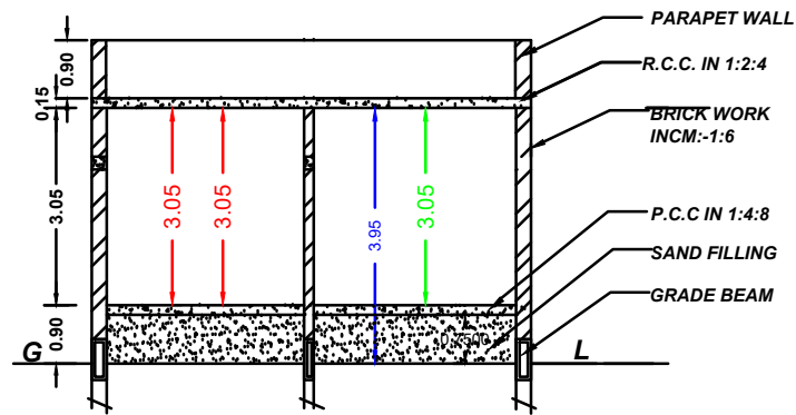
SECTION "AB"
