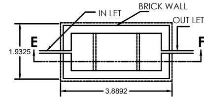
PLAN PLAN OF SEPTIC TANK
