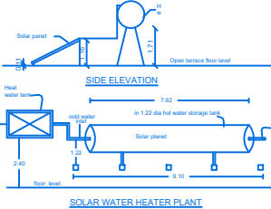
SOLAR WATER HEATER PLANT
