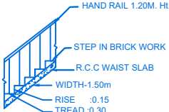
STAIR DETAIL
