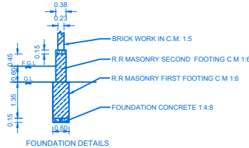
FOUNDATION DETAILS
