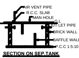
SECTION ON SEPTIC TANK
