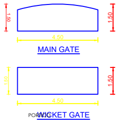
SCALE 1:100
