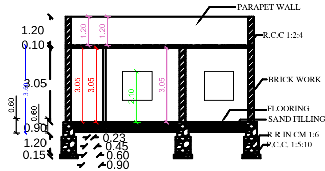
SECTION AB
