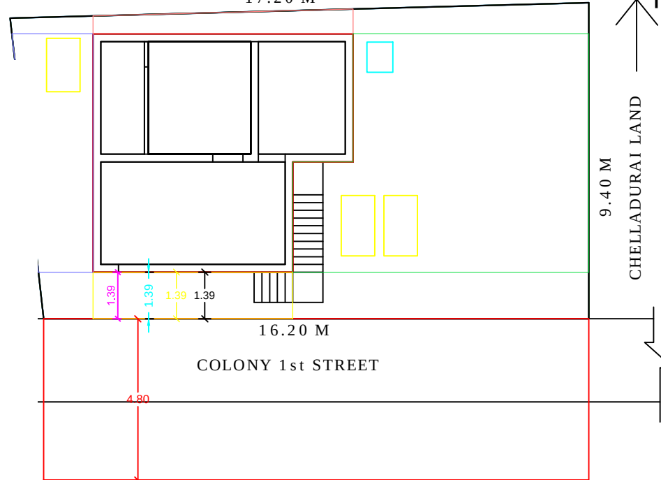
SITE PLAN
