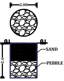
RAINWATER HARVESTING
