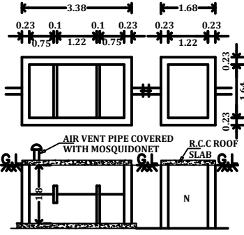
PLAN&SECTION OF SEPTIC TANK 'U' TRAP PROVIDED
