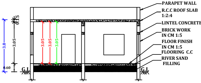
SECTION ON AA1
