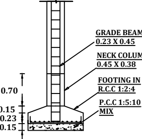
COLUMN DETAILS SCALE - 1:50
