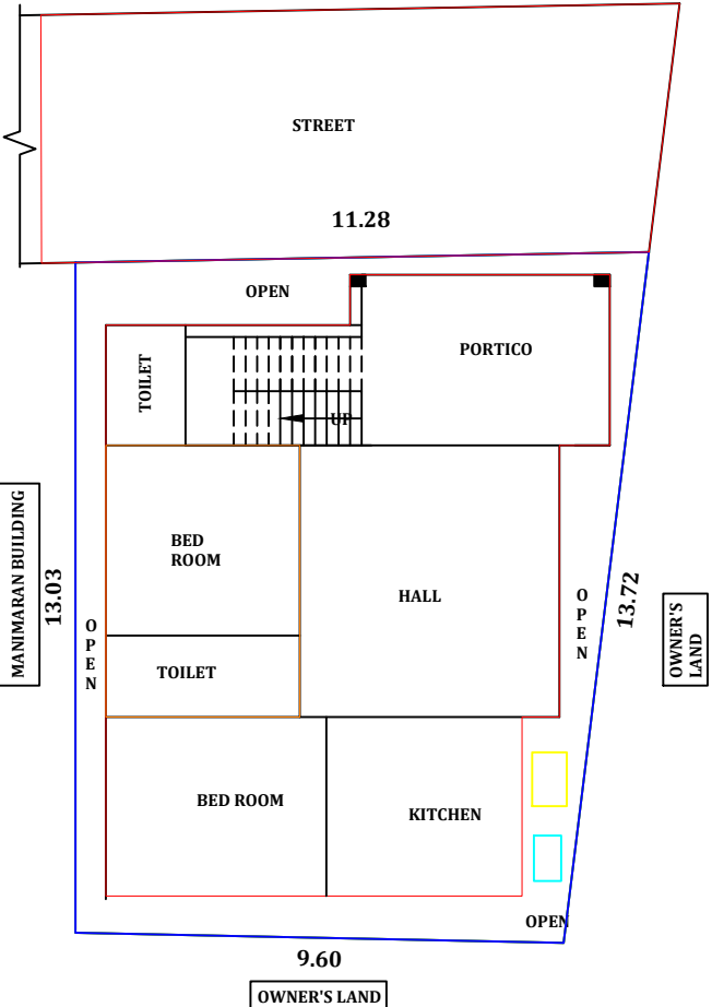
SITE PLAN
