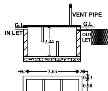
SEPTICTANK DETAILS
