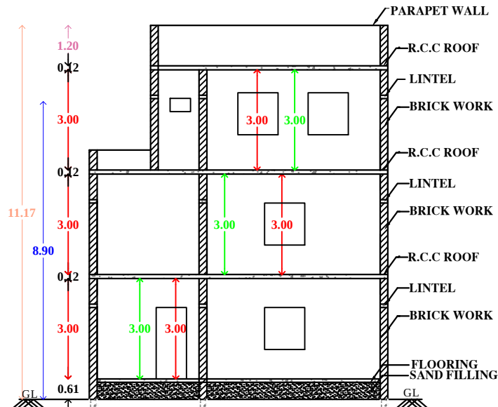
"SECTION "AB"
