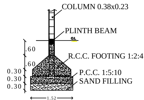
COLUMN DETAILS
