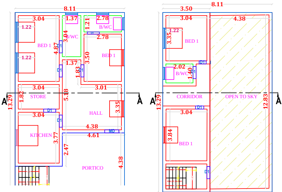
PLAN - FIRST FLOOR PROPOSED
