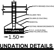
FOUNDATION DETAILS
