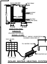
SOLAR WATER HEATING SYSTEM
