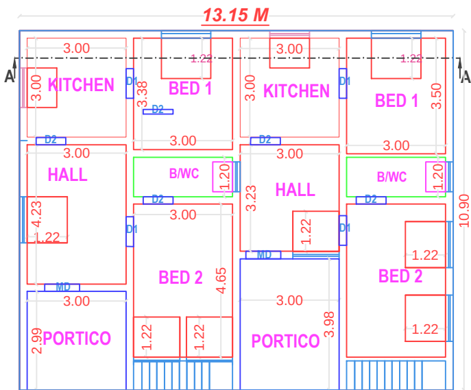
PLAN - GROUND FLOOR (PROPOSED)
