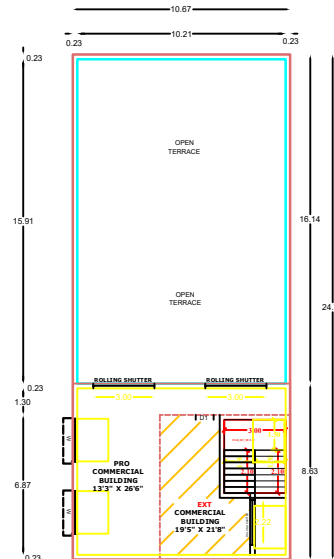
PRO & EXT FIRST FLOOR COMMERCIAL BUILDING PLAN
