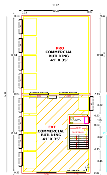
PRO & EXT GROUND FLOOR COMMERCIAL BUILDING PLAN
